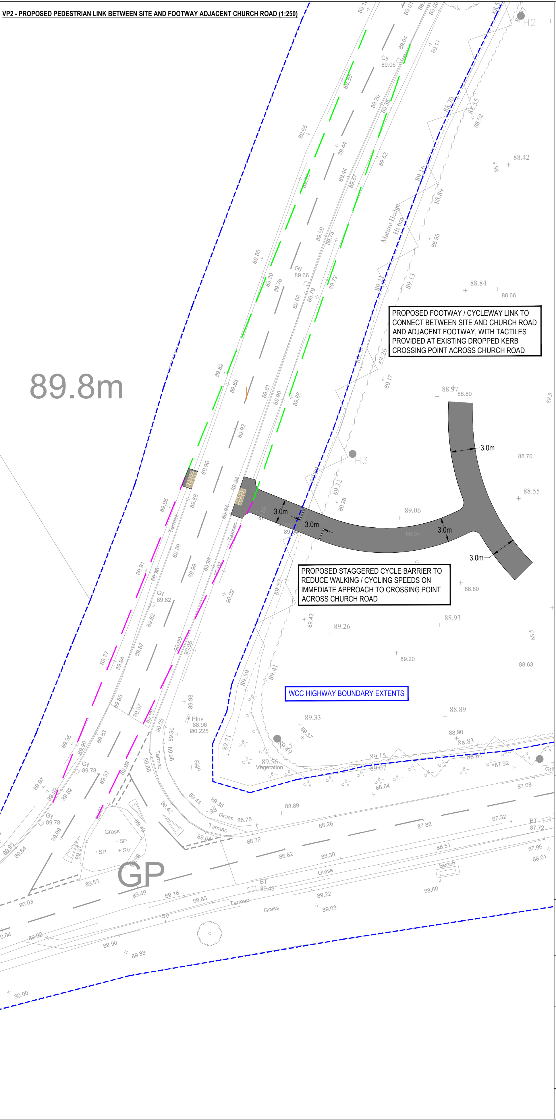
VP2 - PROPOSED PEDESTRIAN LINK BETWEEN SITE AND FOOTWAY ADJACENT CHURCH ROAD (1:250)
