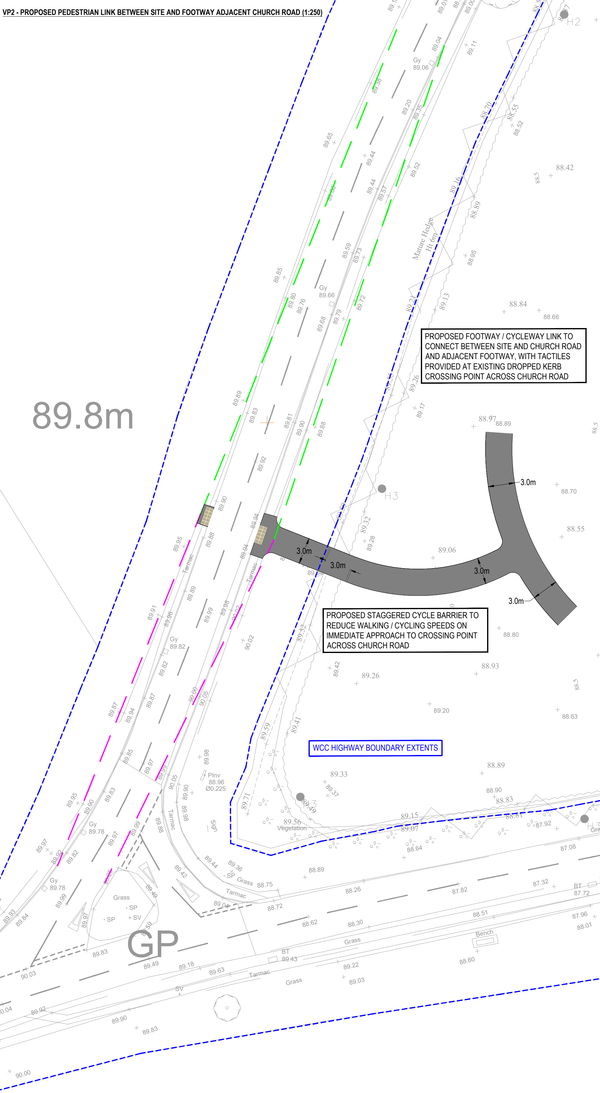
VP2 - PROPOSED PEDESTRIAN LINK BETWEEN SITE AND FOOTWAY ADJACENT CHURCH ROAD (1:250)
