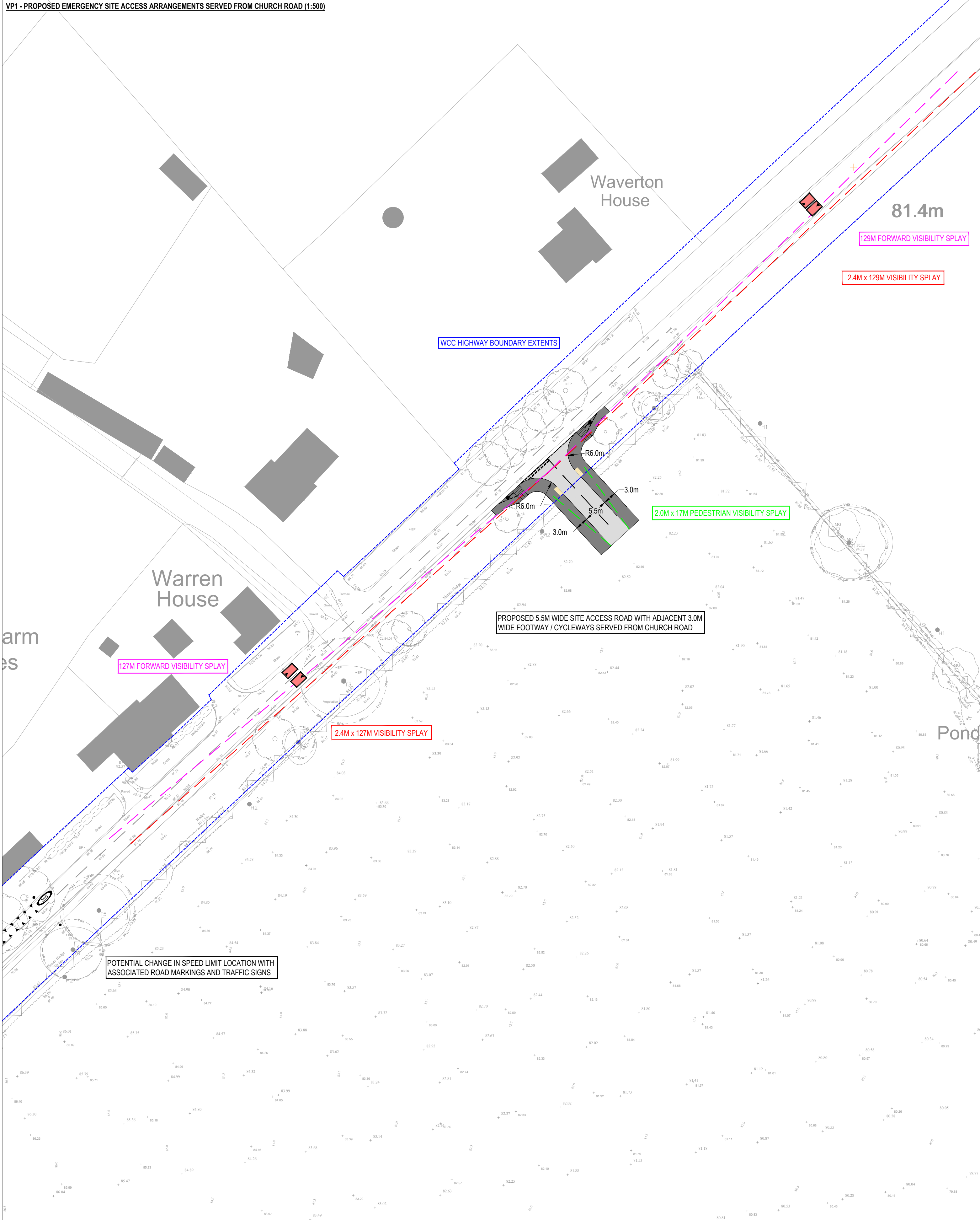
VP1 - PROPOSED EMERGENCY SITE ACCESS ARRANGEMENTS SERVED FROM CHURCH ROAD (1:500)
